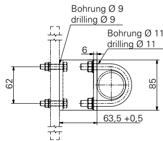
LMHW 48 - FT
