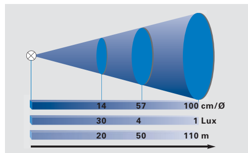
Range-diagram SEB 9 / 8
